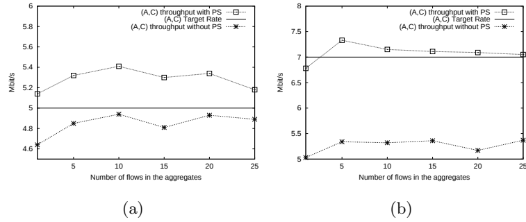
Fig. 8. TCP throughput with various target rates
