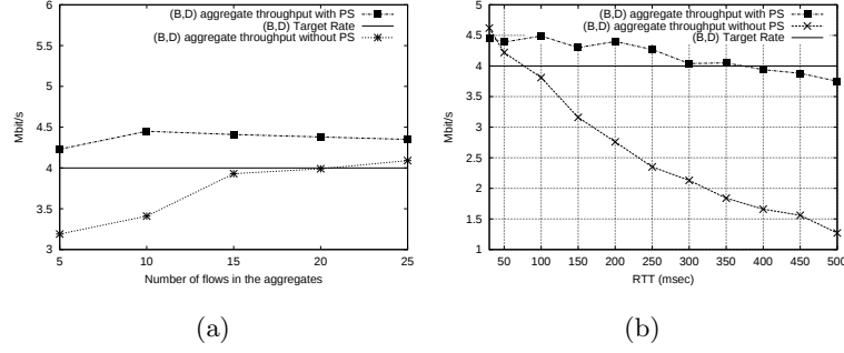
Fig. 9. TCP throughput versus RTT
